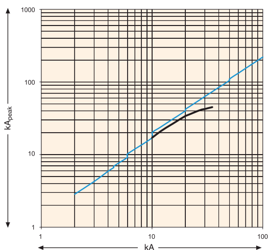
KP 800-F (300-630)A I_{peak} Curve
