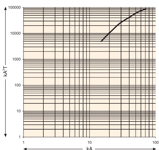
KP 1600-FE I^2T Curve
