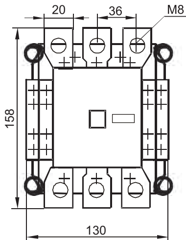
CNKM 80 without IP 20
