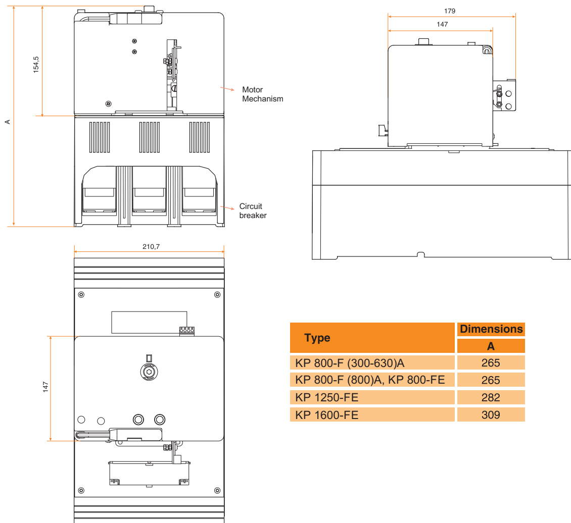
Motor control mechanism for KP 800-F (300-630)A, KP 800-F (800)A, KP 800-FE, KP 1250-FE, KP 1600-FE
