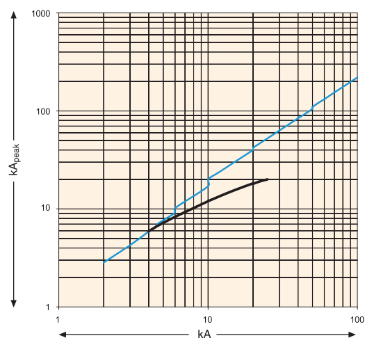
KP 125-F I_{peak} Curve
