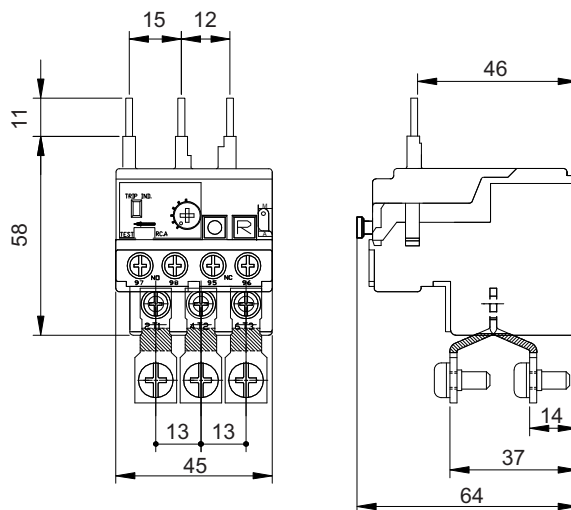
TM 40 with additional terminals
