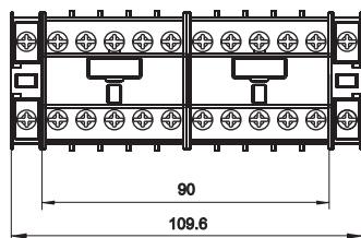
MBCM1 00; MBCM1 11 MBCM1..N 00; MBCM1..N 11
