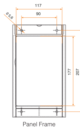
Panel Frame
