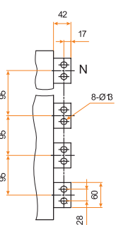
Busbar Connections
