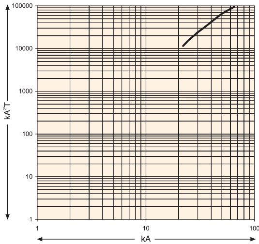
KP 2500-FE I^2T Curve
