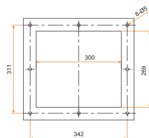
Panel Frame
