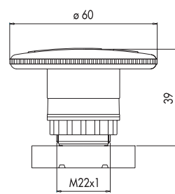
Emergency Stop Ø 60 mm
