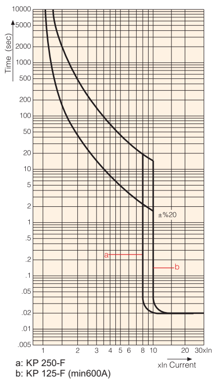
KP 125-F - KP 250-F Thermal magnetic circuit breakers
