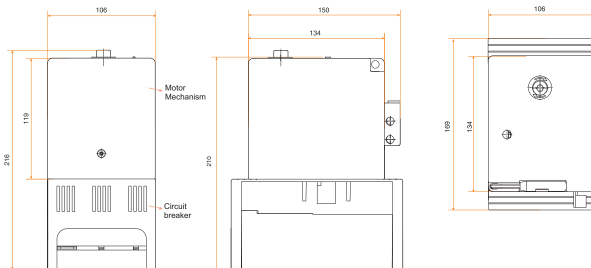
Motor control mechanism for KP 250-F
