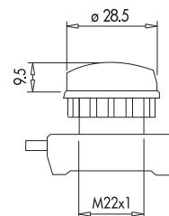
Pilot Light
