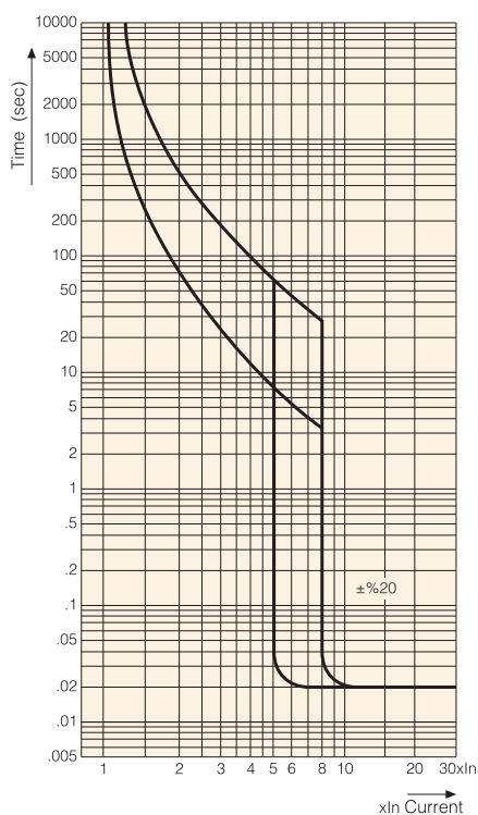
KP 800-F (800A) Thermal magnetic circuit breakers
