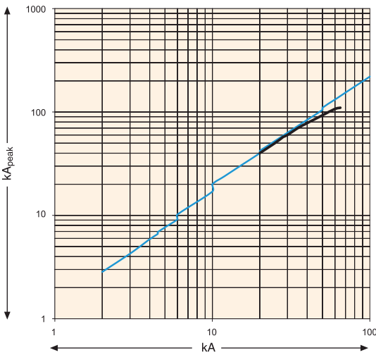
KP 2500-FE I_{peak} Curve
