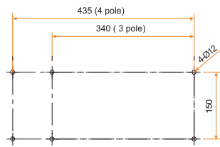
Assembling Gauge
