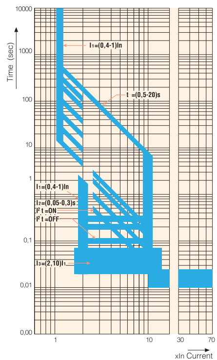
KP 800-FE - KP 2500-FE Electronic circuit breakers
