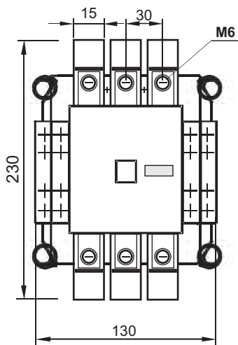
CNKM 80 with IP 20
