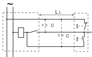
Control with push button
