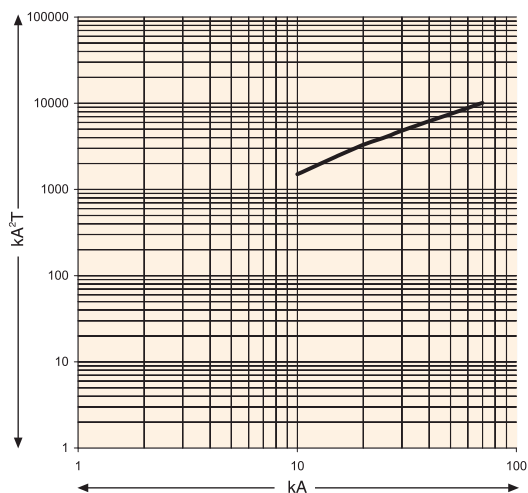
KP 800-F (800)A/KP 800-FE I^2T Curve
