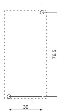
Drilling plan
