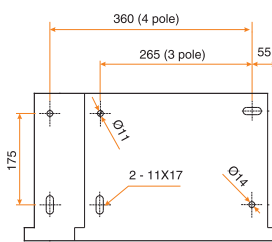
Assembling Gauge
