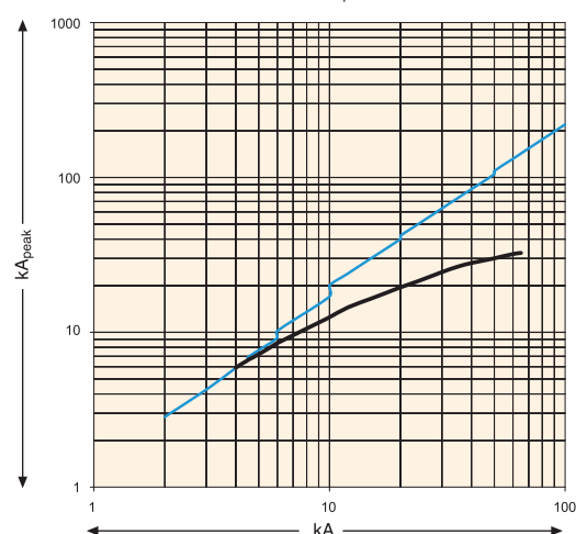
KP 250-F I_{peak} Curve
