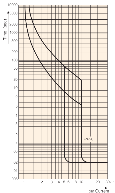
KP 800-F (300-630A) Thermal magnetic circuit breakers
