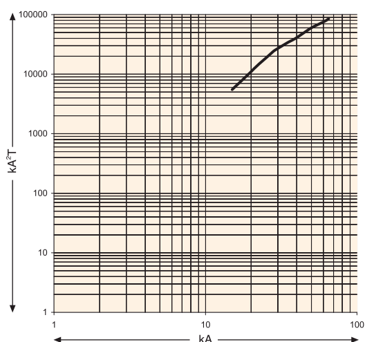
KP 1250-FE I^2T Curve
