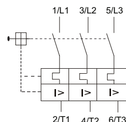
Schematic diagram DMS 25
