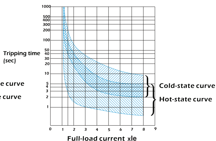
Three-phase protection characteristics
