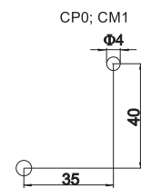
Drilling plan (mm)
