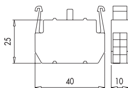
Contact Block
