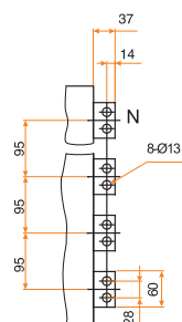
Busbar Connections
