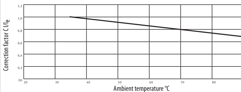
Influence of ambient temperature on rated current of NH strip-type fuse-switch-disconnectors
